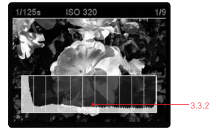
3.3.2 DNG-Histogram
